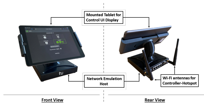
Fig. 3. Physical realization of the vSTING module, comprised of an embedded computer for network emulation and a mounted tablet to display the UI controls.
