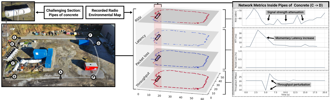
Fig. 8. Scenario setup for the network replay evaluation: The outdoor test field scenario of the German Rescue and Robotics Center furnished with Wi-Fi connectivity. The obstacles present in the field yield effects on the observed connectivity, especially when the robot moves through the pipe system at the left edge. This specific part of the metrics was taken for evaluating the network replay functionality.
