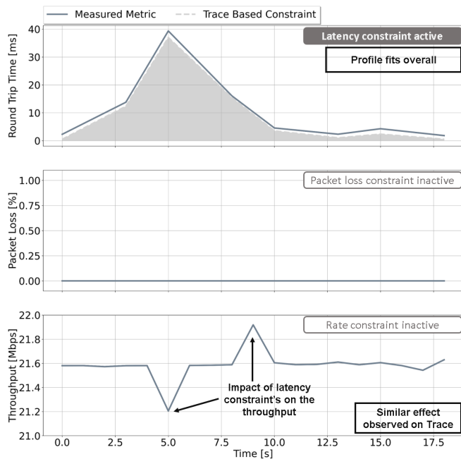
Fig. 9. Network replay while using only the latency traces as constraint. The generated metrics for the latency match the recorded trace profile. The throughput shows a similar trend to the traces in response to latency fluctuations.
