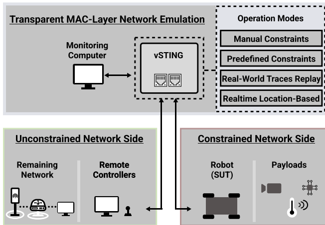
Fig. 2. Concept for the encapsulation of network constraints in a module: Network emulation applied on transparently forwarded traffic by the module.
