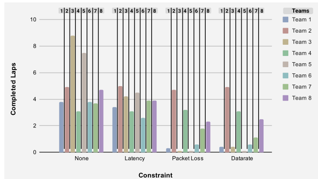
(a) Absolute Teleoperation Performance.
