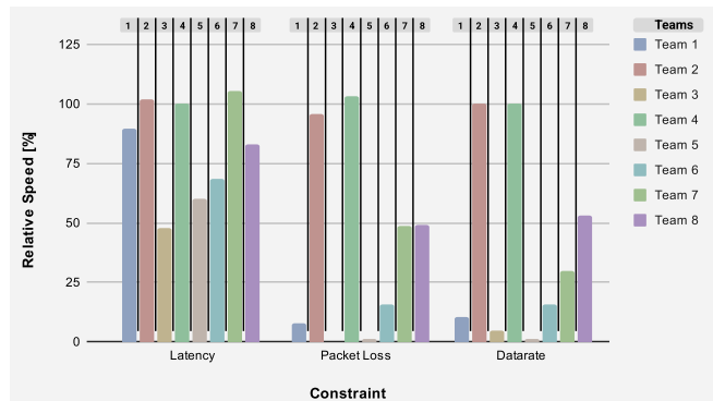
(b) Teleoperation Performance relative to unconstrained run.
