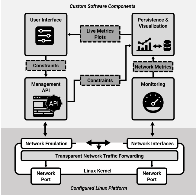
Fig. 4. Logical architecture running on the hardware of the vSTING module. The developed additions run atop the Linux kernel’s network emulation applied on the forwarded network traffic.
