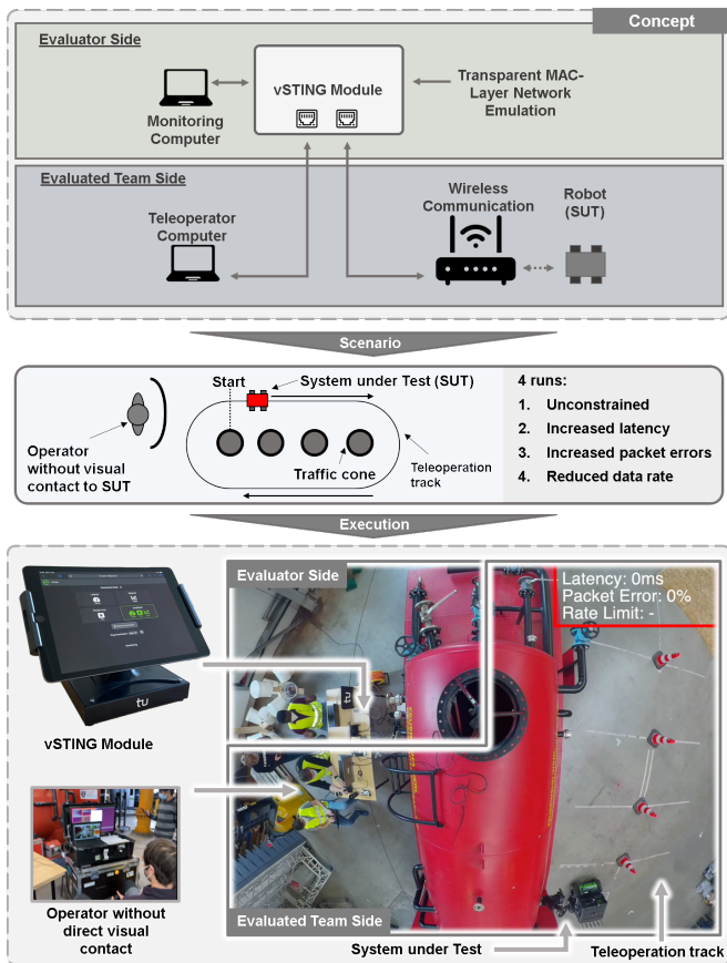
Fig. 6. Setup for evaluating the teleoperation performance under network constraints. The robot operator must complete as many laps as possible on the defined course during multiple three minutes runs with different vSTING-enabled network constraints.
