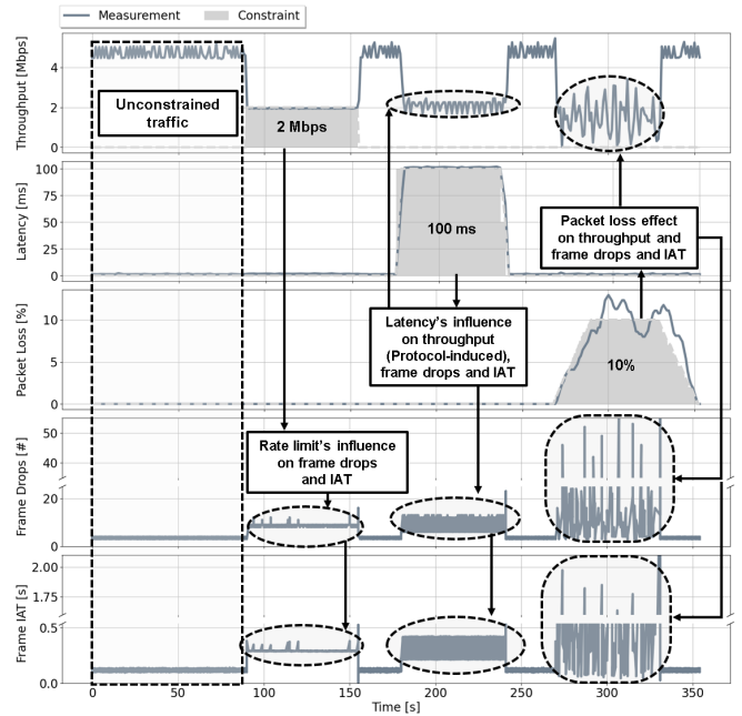
Fig. 5. Manual enforcement of constraints on live traffic of a robot’s FPV Camera. The physical dependencies between the network metrics and protocol-induced cross-metrics effects can be observed. Frames drops and Inter Arrival Time (IAT) also monitored, to capture the constraints’ effect on the FPV stream.
